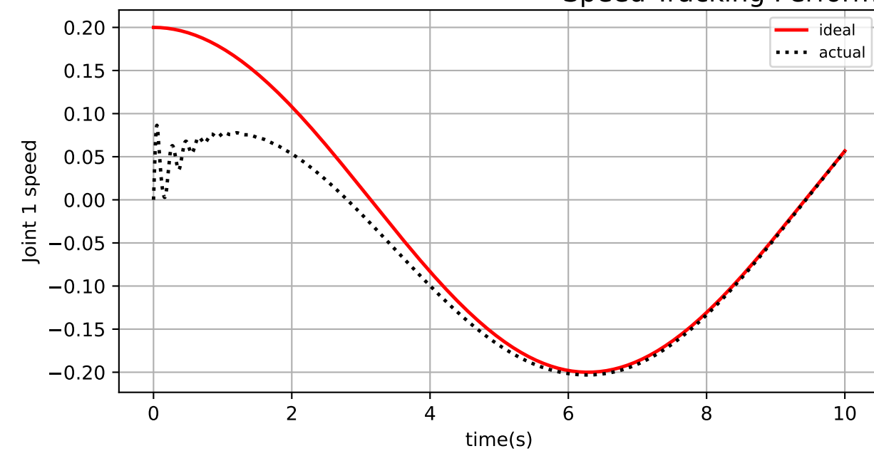
Speed Tracking Performance ( S=3 , S1=2 , m=19 )
