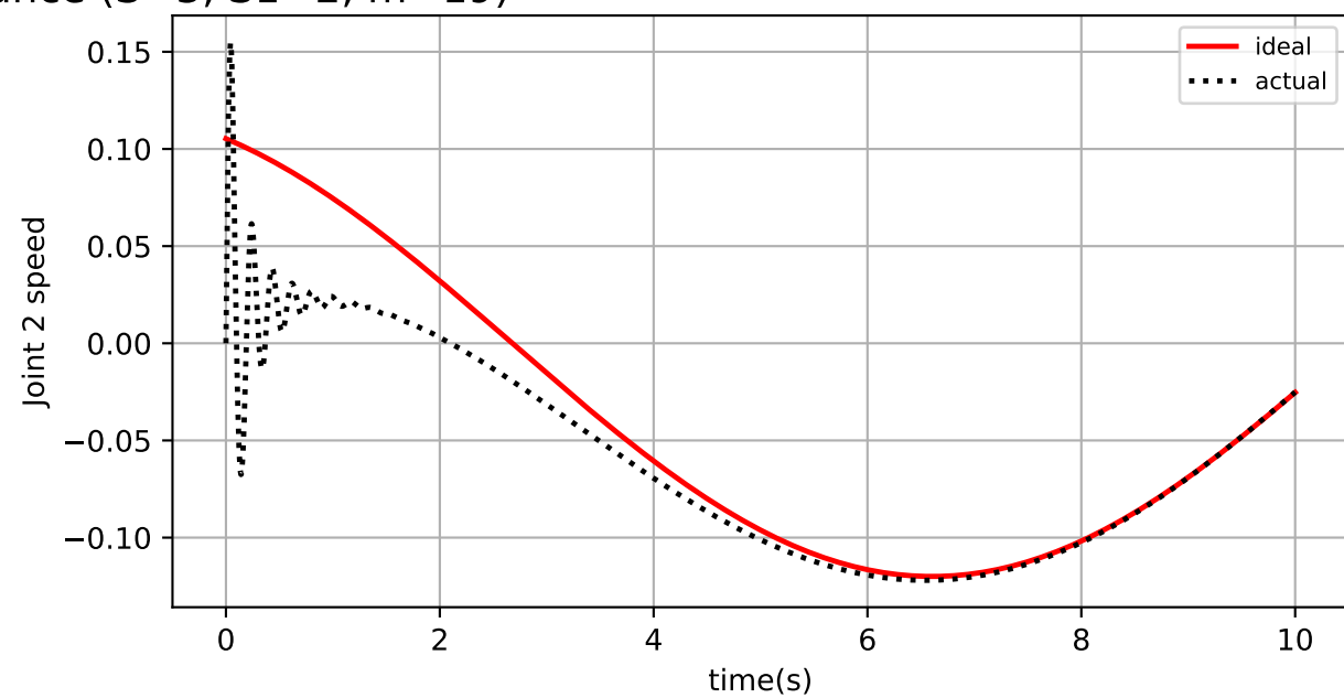
Speed Tracking Performance ( S=3 , S1=2 , m=19 )
